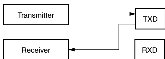
Figure 20-30. Single-Wire Operation (LOOPS = 1, RSRC = 1)
