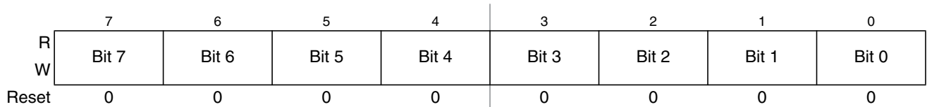
Figure 14-25. Timer Input Capture/Output Compare Register 2 Low (TC2)
